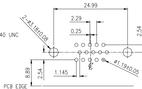
RECOMMENDED P.C.B LAYOUT (VIEW FROM TOP SIDE)
